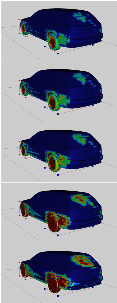
Fig. 6. Steps 1 to 5 of a soiling simulation running for approximately 24 hours on a dual processor SGI Octane MXI with 2x250MHz MIPS R10K. The colorcoding shows the hit rate of particles colliding with the car body. Red hot spots indicate areas with a high degree of soiling.
