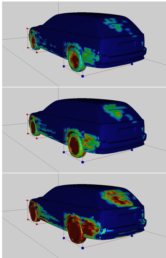
Steps 1 to 3 of a soiling simulation running for approximately 24 hours on a dual processor SGI Octane MXI with 2x250MHz MIPS R10K. The colorcoding shows the hit rate of particles colliding with the car body. Red hot spots indicate areas with a high degree of soiling.
